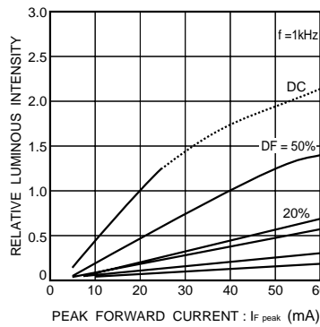
Fig. 18 Luminous intensity vs. peak forward current
