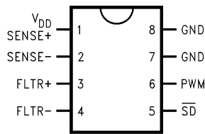
Top View LM3812 for High-Side Sensing
