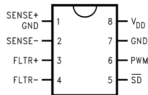
Top View LM3813 for Low-Side Sensing
