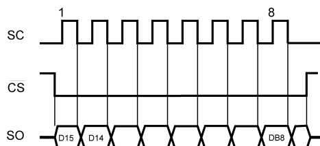
a) Reading Continuous Conversion - Single Eight-Bit Frame
