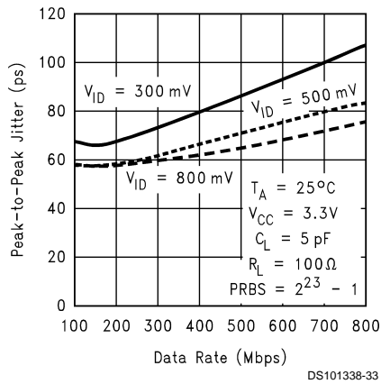
Peak-to-Peak Output Jitter at V_CM = 0.4V vs Differential Input Voltage
