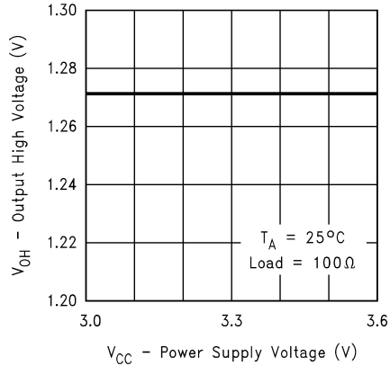
Output High Voltage vs Power Supply Voltage
