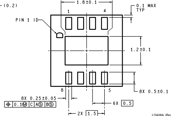
Order Number DS90LV001TLD See NS Package Number LDA08A
