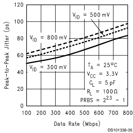
Peak-to-Peak Output Jitter at V_CM = 2.9V vs Differential Input Voltage
