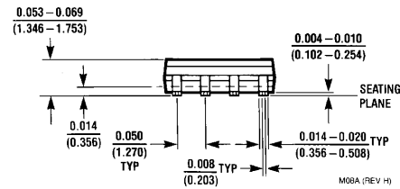
Order Number DS90LV001TM See NS Package Number M08A
