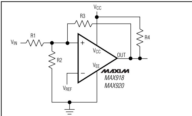
Figure 4. MAX918/MAX920 Additional Hysteresis
