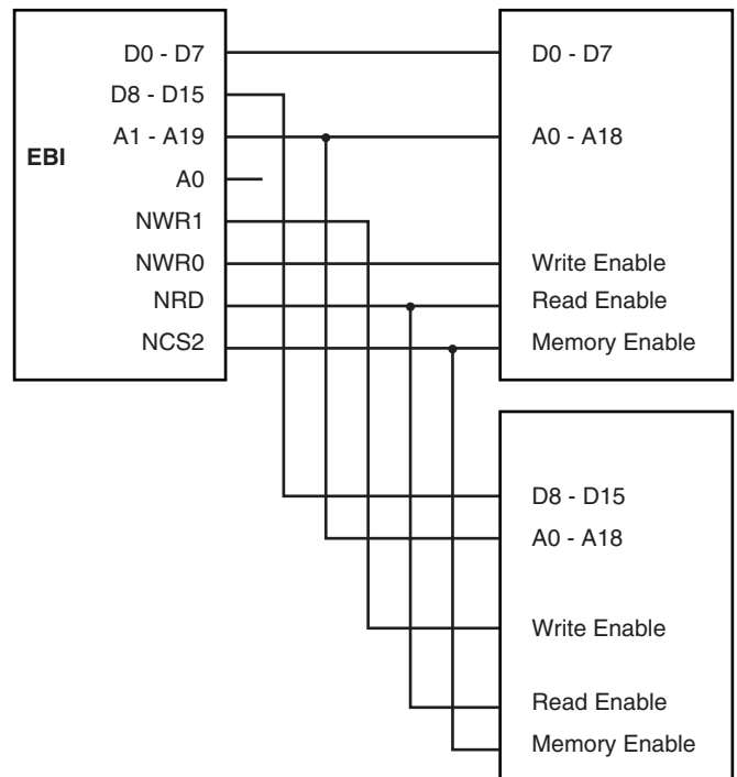
Figure 11. Memory Connection for 2 x 8-bit Data Busses
