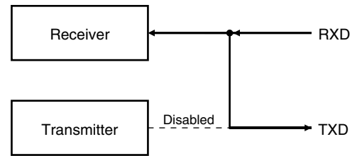
Figure 42. Channel Modes
