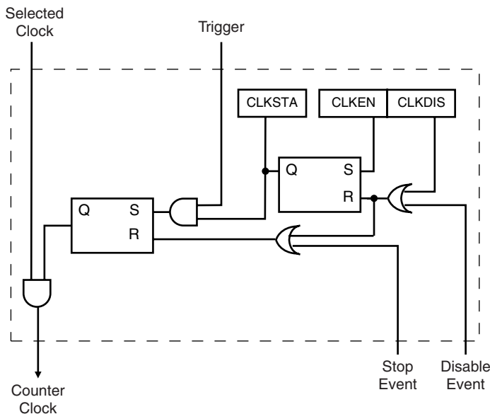
Figure 45. Clock Control
