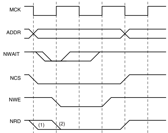
Figure 20. External Wait
