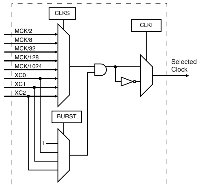
Figure 44. Clock Selection
