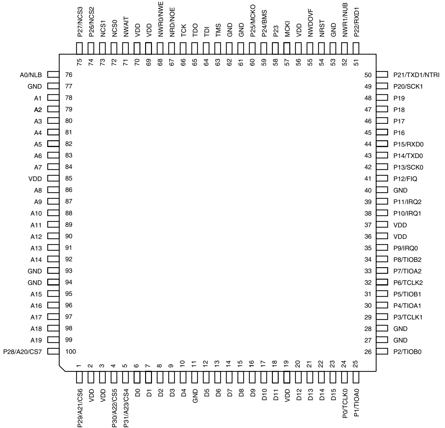
Figure 1. AT91X40 Series Pinout (Top View)
