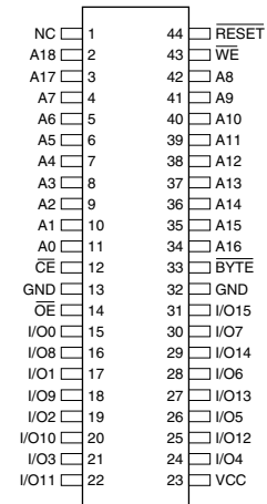
AT49F8192A(T) SOIC (SOP) Top View
